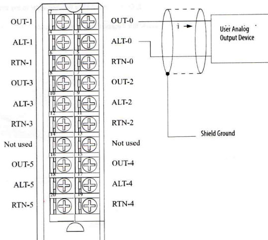
Figure 46 - 1756-OF6CI Wiring Example for Loads of 551-1000 \Omega
