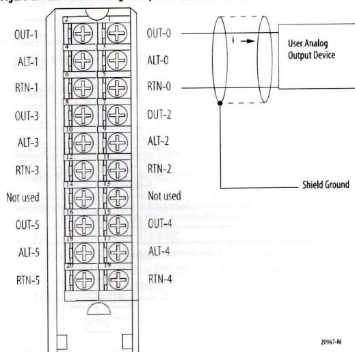
Figure 45 - 1756-OF6CI Wiring Example for Loads of 0-550 \Omega
