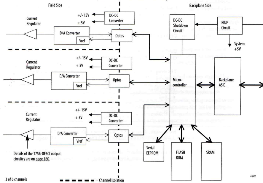
Figure 41 - 1756-OF6CI Module Block Diagram
