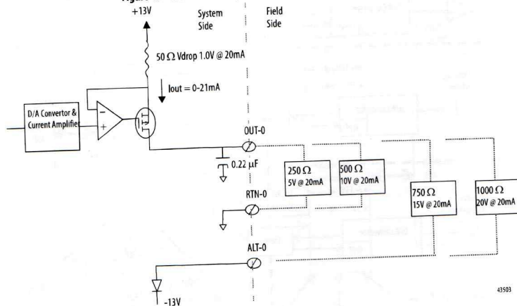
Figure 43 - 1756-OF6CI Output Circuit
