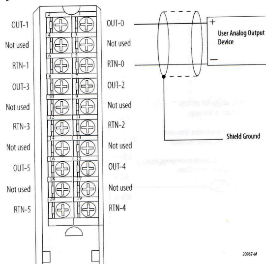
Figure 47 - 1756-OF6VI Wiring example
