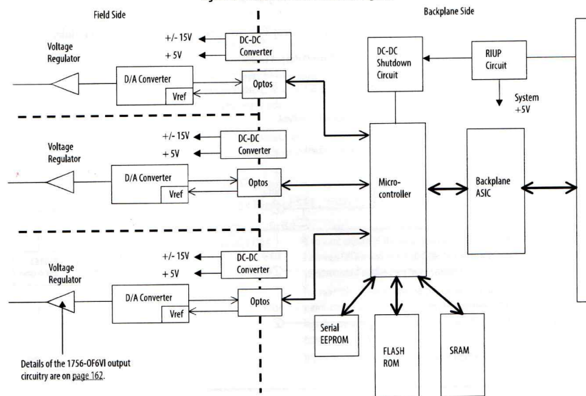
Figure 42 - 1756-OF6VI Module Block Diagram
