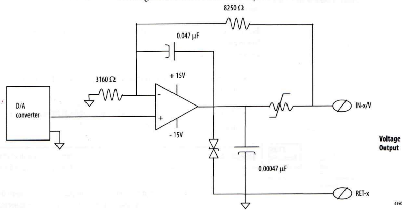
Figure 44 - 1756-OF6VI Output Circuit
